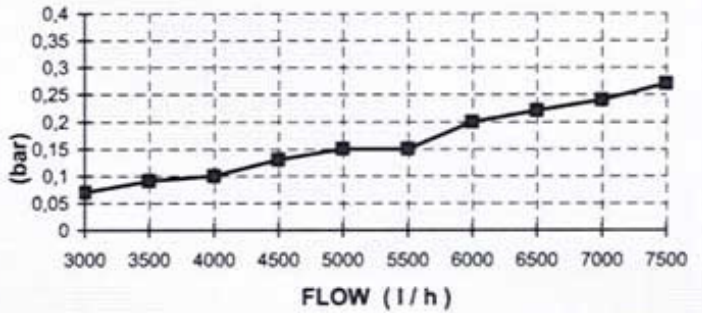
SLEEVE 10 µm
