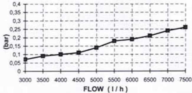
SLEEVE 25 µm
